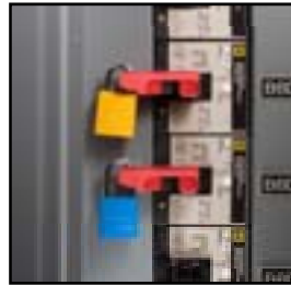
Electrical lockout
